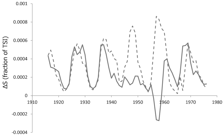
Figure 3. A plot of the annual means of \Delta S for 1916–1976 reconstructed from A_f (solid) and from A_{pn} (dashed).
