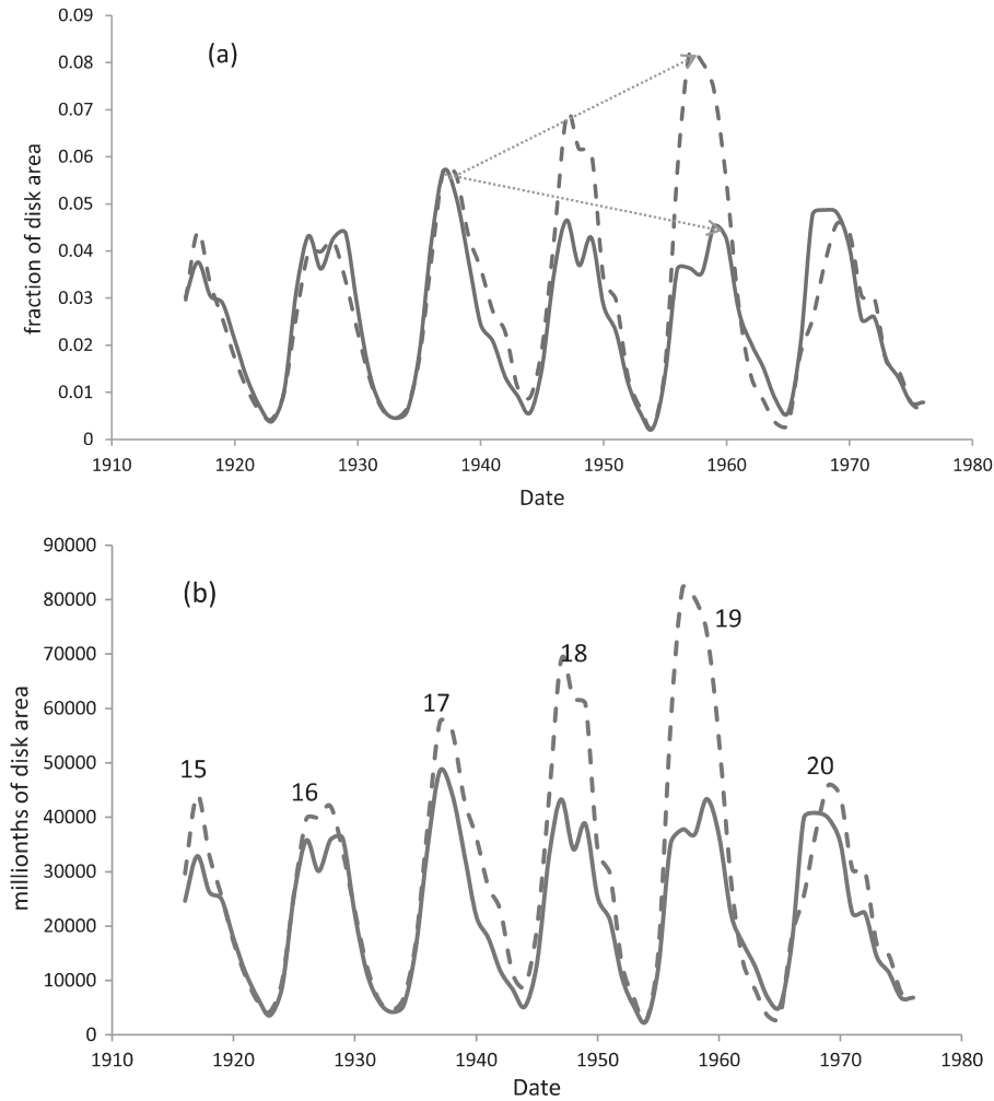
Figure 2. (a) The annual mean A_f (solid) and A_{pn} for sunspot cycles 15–20. A_f has been multiplied by 20. The arrows show the trends of peak A_{pn} and A_f . Panel (b) shows the observed (dashed) and calculated (solid) A_{pn} from relation (1).
