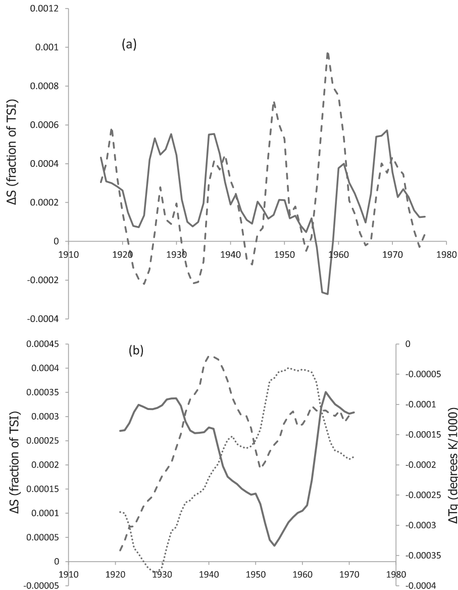
Figure 4. (a) Comparison of \Delta S from A_f (solid) and the NRL TSI time series (dashed); (b) 11-year smoothed \Delta S from A_f (solid), NRL (dotted) compared to the global temperature variation, T_g (dashed).
