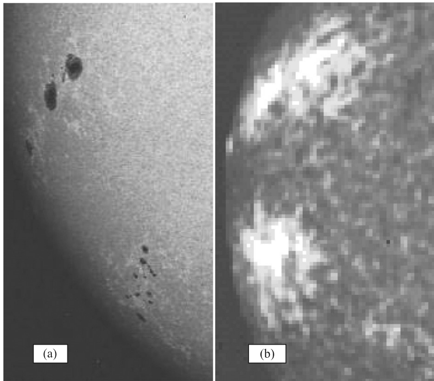
Figure 1. (a) The solar disk imaged in photospheric broadband light and (b) in chromospheric Ca K radiation. WL faculae are seen around the spots in (a); Ca K plages cover them and also most of the sunspots, in (b). Images obtained at Mt. Wilson Observatory on 1957 September 15.
